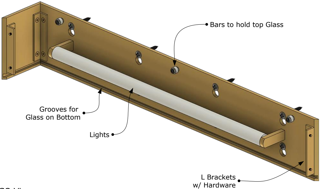
ISO View (Plates and Glass Removed)
