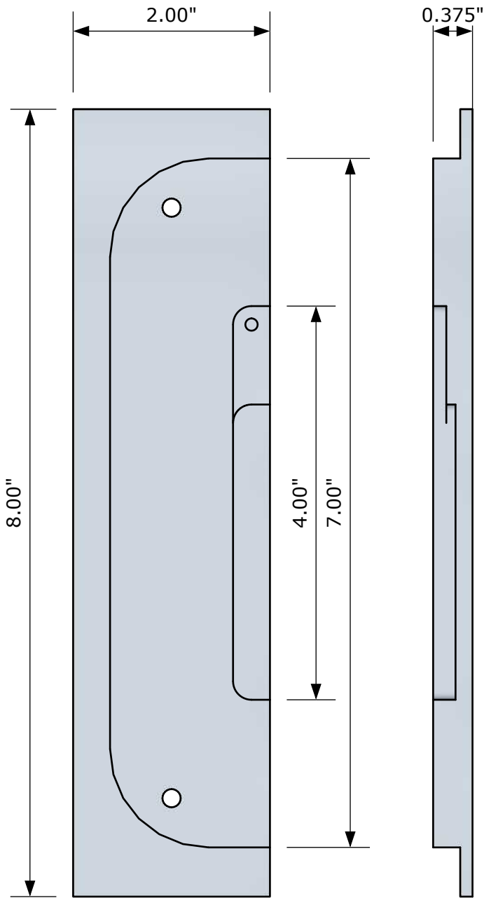
Back View
