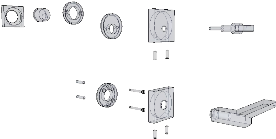
EXPLODED VIEW
